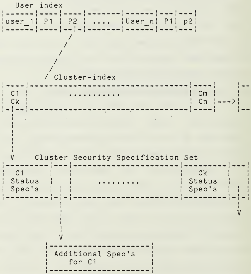
Figure 3.9 The Secondary-Storage-Based CSST
